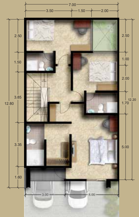
2nd Floor
