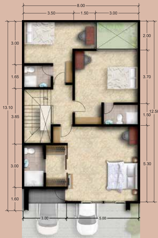
2nd Floor
