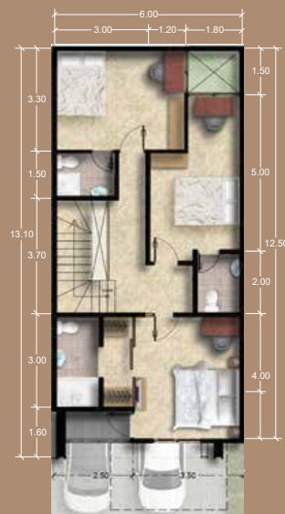
2nd Floor
